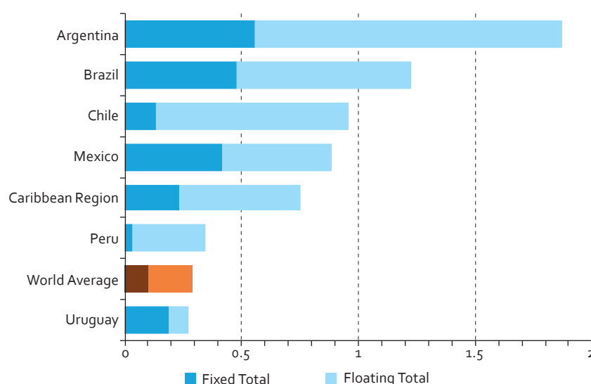
Figure XII.1 Technical potential for offshore wind generation in Latin America and the Caribbean
