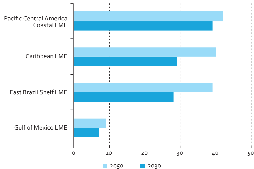
Figure IV.1 Projections of coral reef risk for years 2030 and 2050 due to ocean acidification (Percentages)
