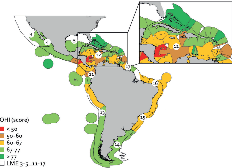
Map III.1 Ocean Health Index of Latin American and Caribbean Large Marine Ecosystems (2019)
